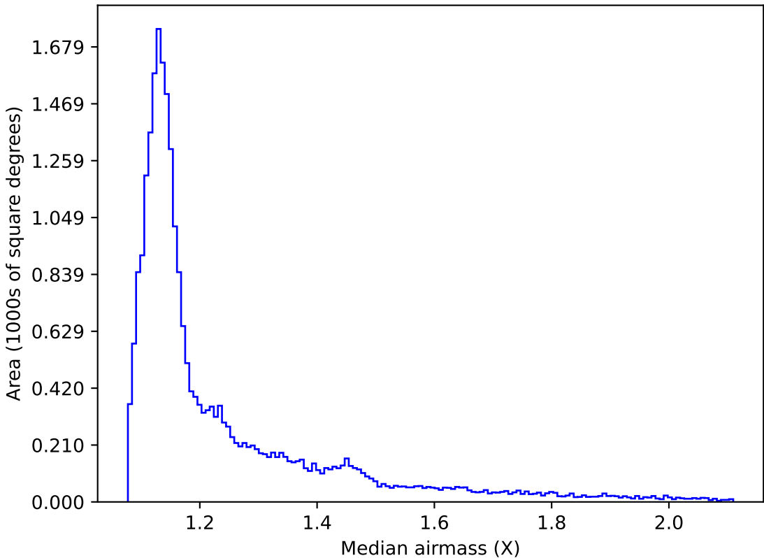
roll_pause_mjdp120_v3.4_10yrs All sky i band: Median airmass
