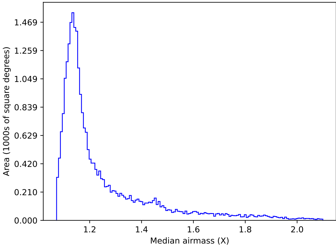
roll_pause_mjdp120_v3.4_10yrs All sky g band: Median airmass
