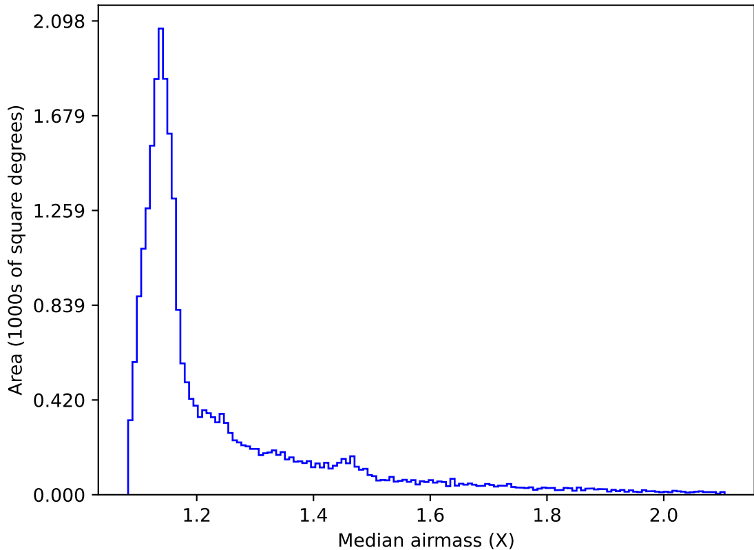
roll_pause_mjdp120_v3.4_10yrs All sky all bands: Median airmass
