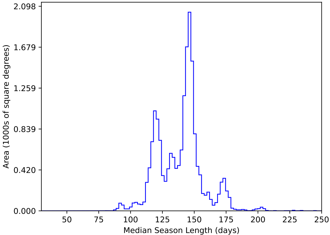
roll_pause_mjdp120_v3.4_10yrs WFD y band: Median Season Length
