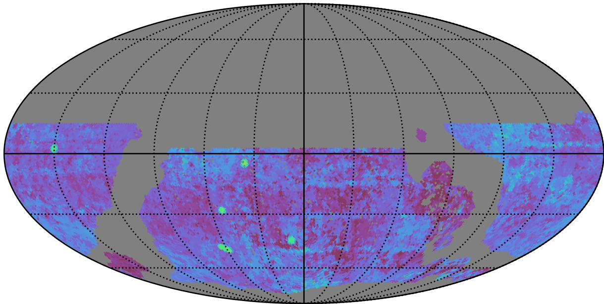
roll_pause_mjdp120_v3.4_10yrs WFD u band: Median Season Length
