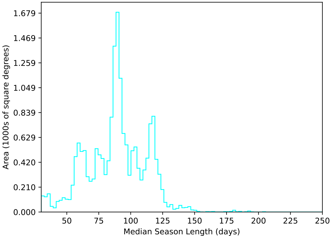
roll_pause_mjdp120_v3.4_10yrs WFD u band: Median Season Length
