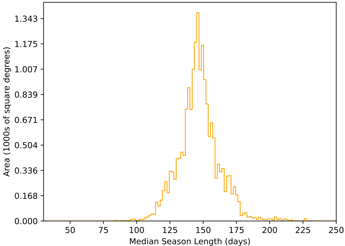
roll_pause_mjdp120_v3.4_10yrs WFD r band: Median Season Length
