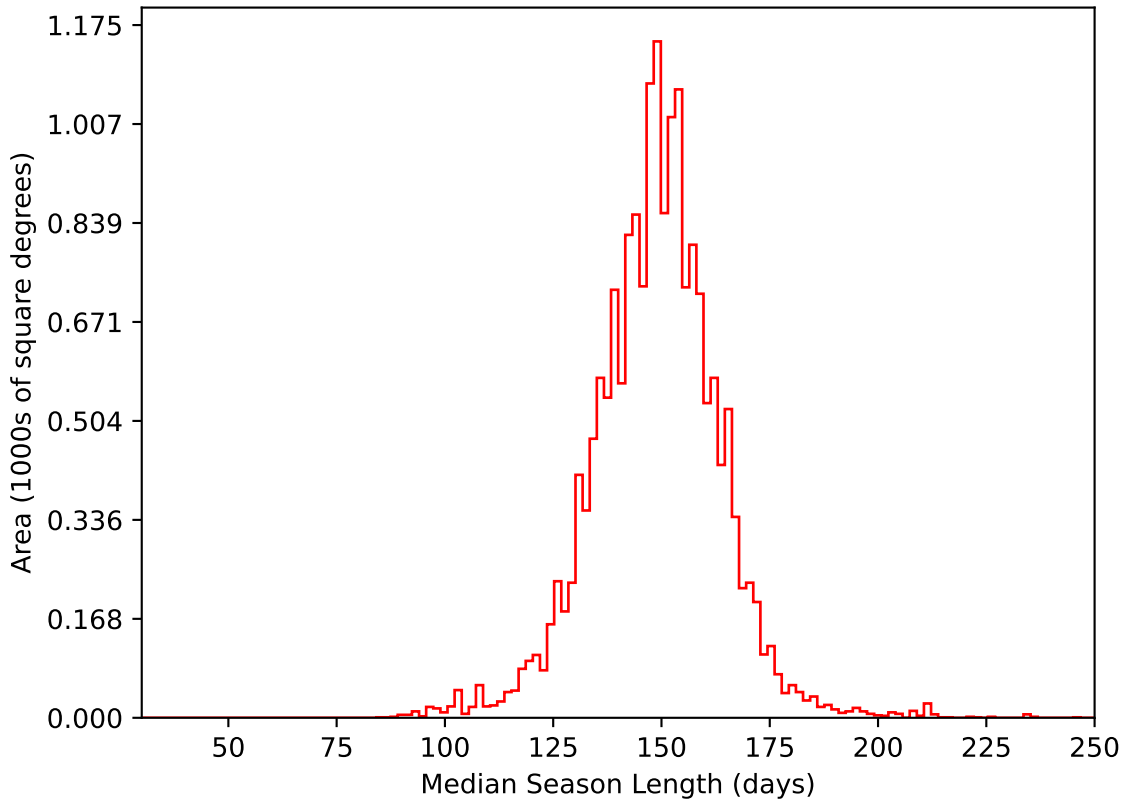
roll_pause_mjdp120_v3.4_10yrs WFD i band: Median Season Length
