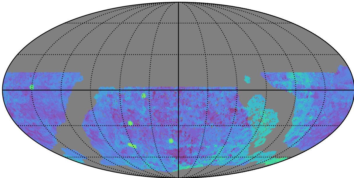
roll_pause_mjdp120_v3.4_10yrs WFD g band: Median Season Length
