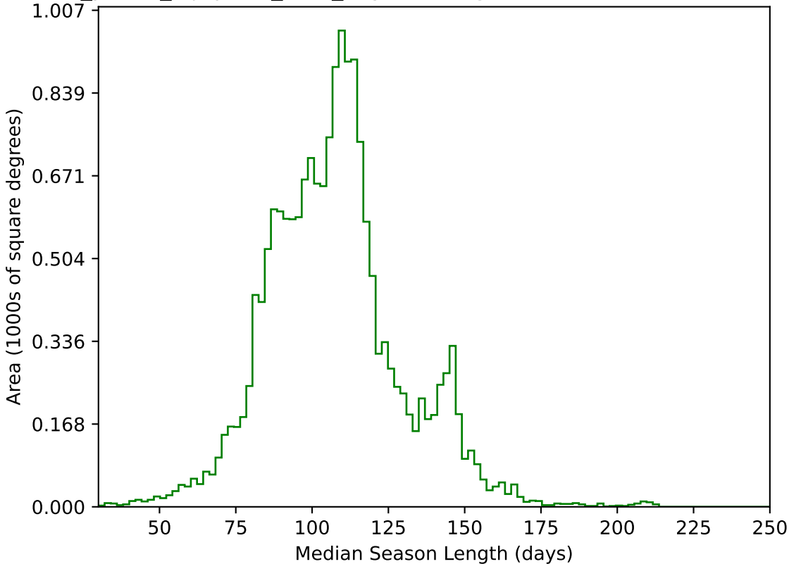
roll_pause_mjdp120_v3.4_10yrs WFD g band: Median Season Length
