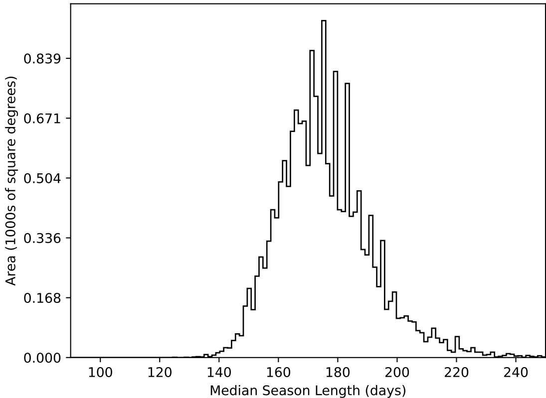
roll_pause_mjdp120_v3.4_10yrs WFD all bands: Median Season Length
