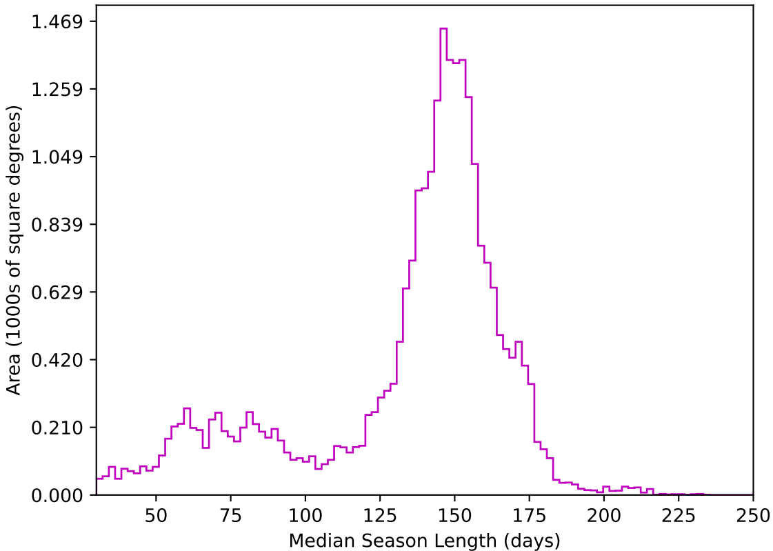
roll_pause_mjdp120_v3.4_10yrs All sky z band: Median Season Length
