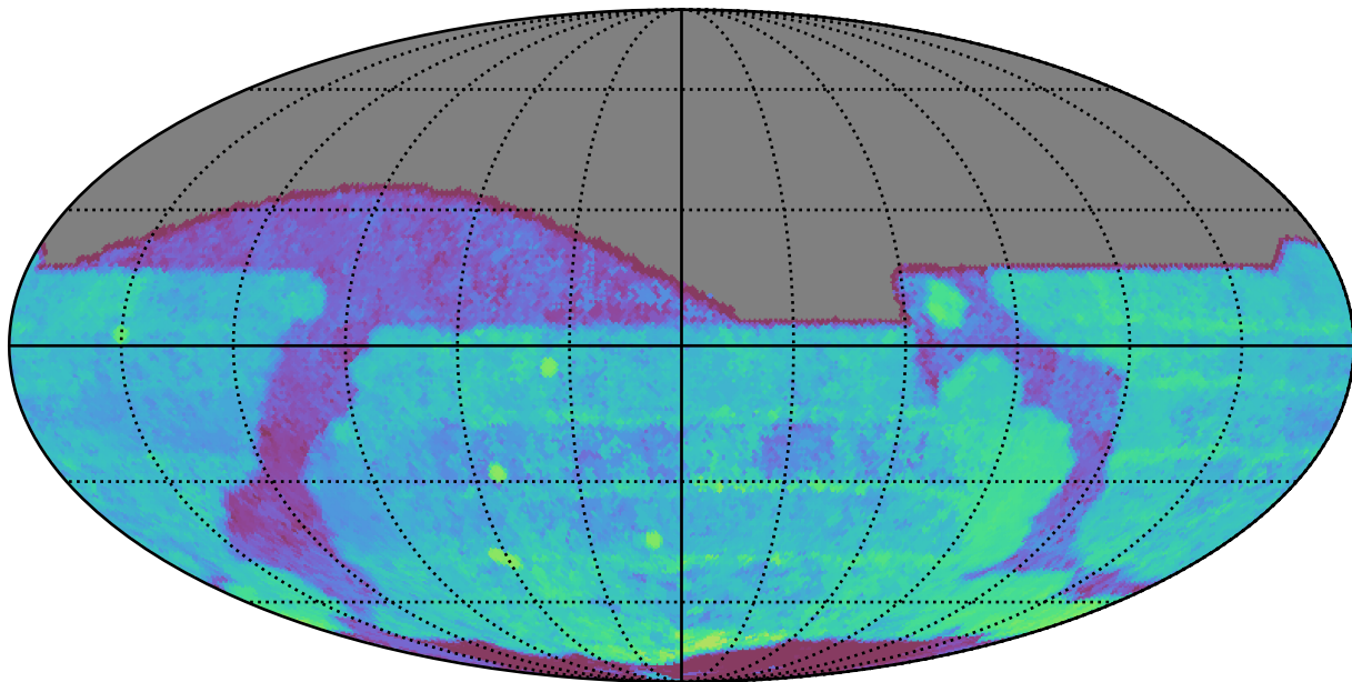
roll_pause_mjdp120_v3.4_10yrs All sky r band: Median Season Length
