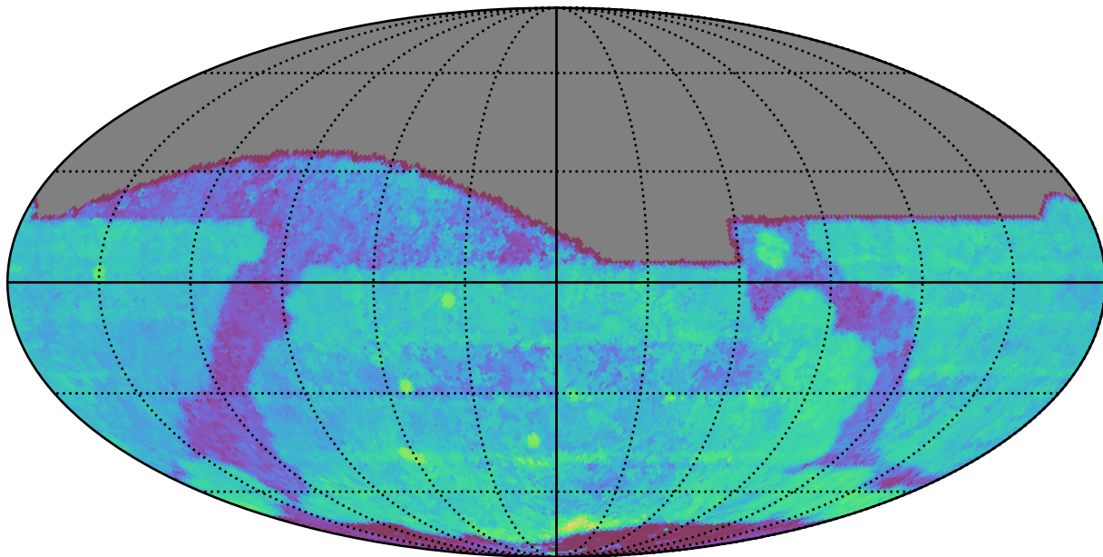
roll_pause_mjdp120_v3.4_10yrs All sky i band: Median Season Length
