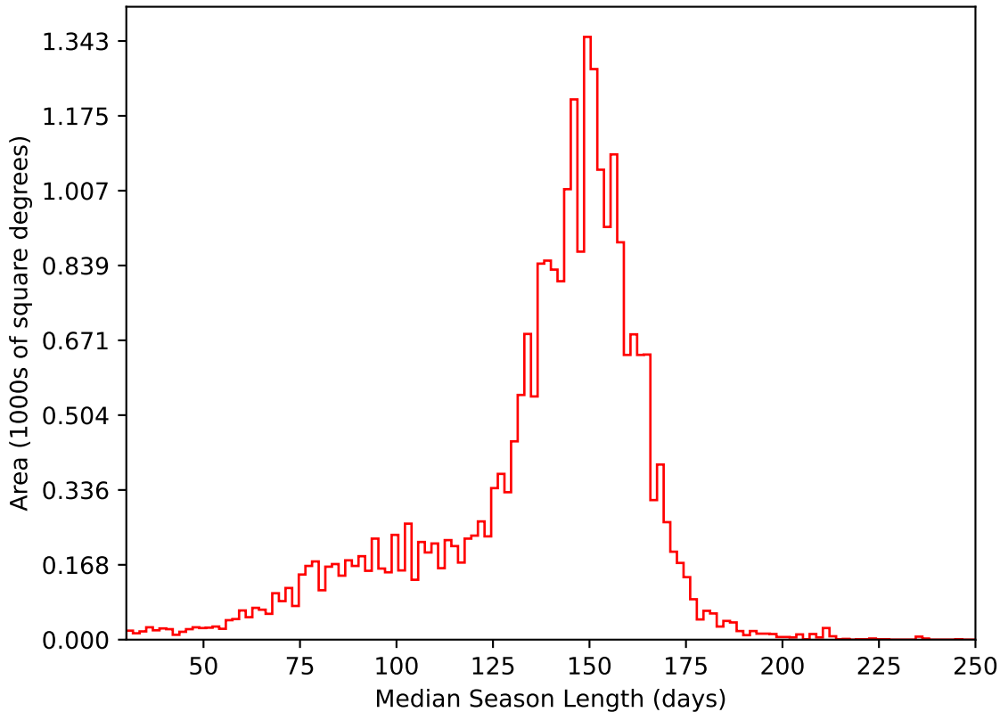
roll_pause_mjdp120_v3.4_10yrs All sky i band: Median Season Length
