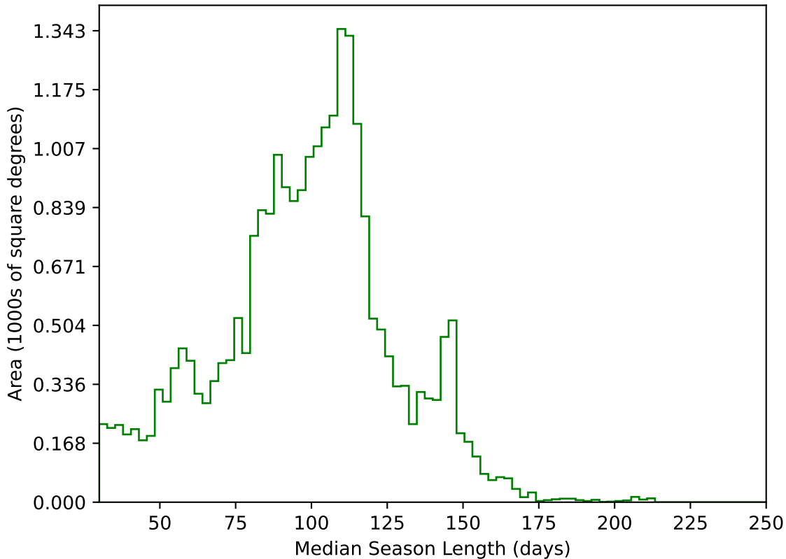
roll_pause_mjdp120_v3.4_10yrs All sky g band: Median Season Length
