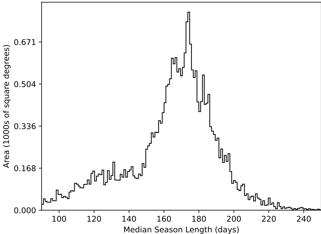
roll_pause_mjdp120_v3.4_10yrs All sky all bands: Median Season Length
