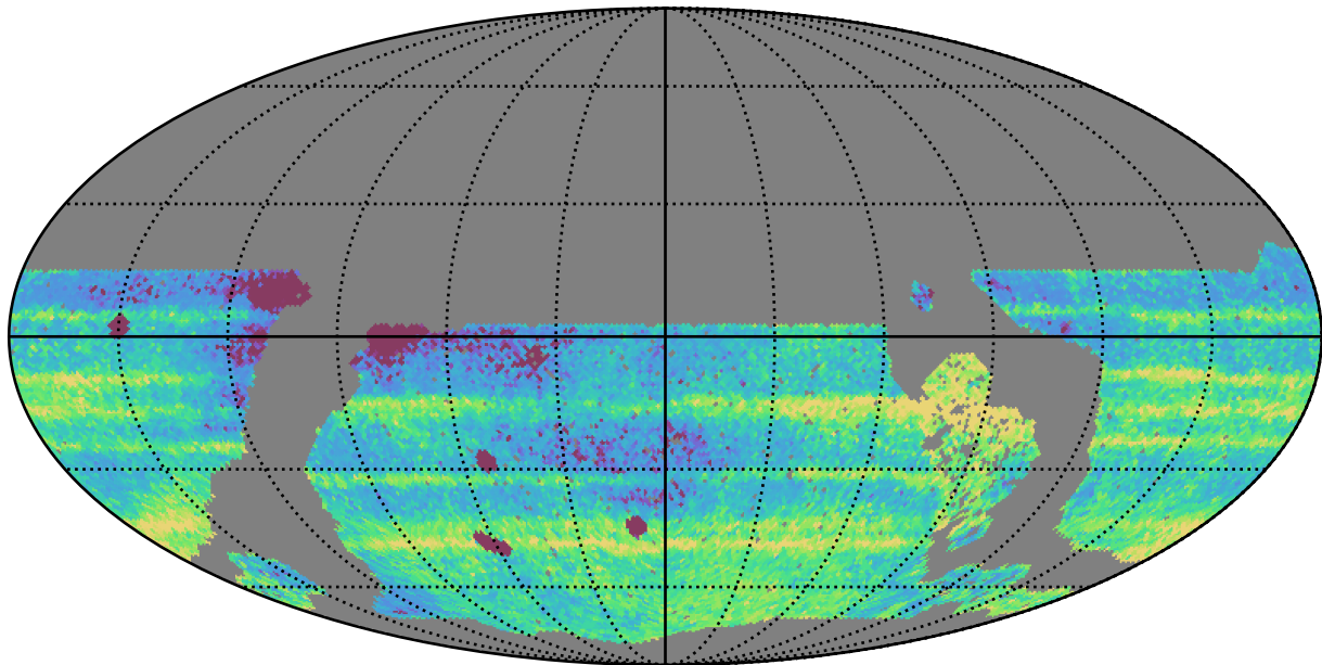
roll_pause_mjdp120_v3.4_10yrs WFD: Median Intra-Night Gap
