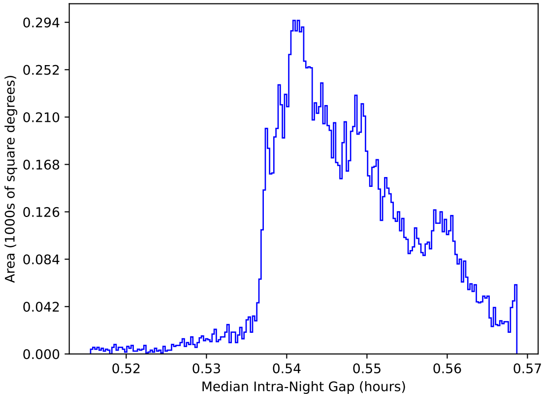
roll_pause_mjdp120_v3.4_10yrs WFD: Median Intra-Night Gap
