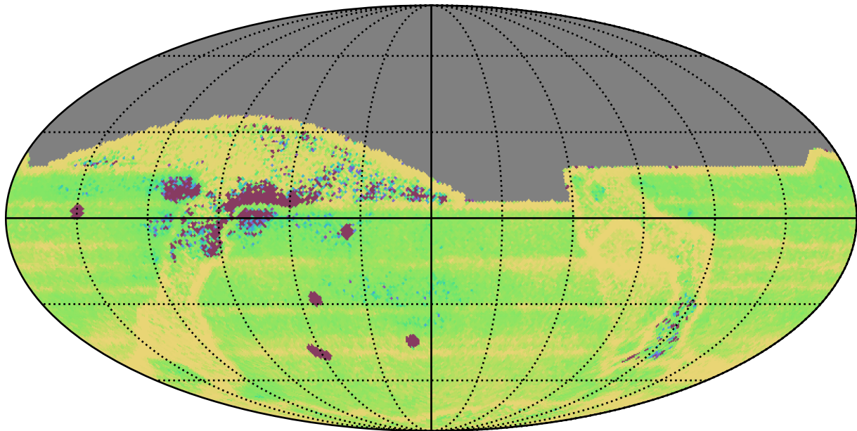
roll_pause_mjdp120_v3.4_10yrs All sky: Median Intra-Night Gap
