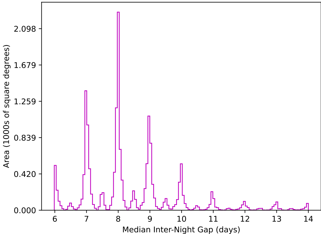
roll_pause_mjdp120_v3.4_10yrs WFD z band: Median Inter-Night Gap
