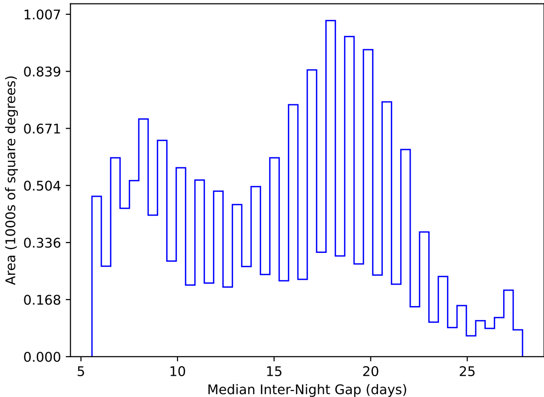
roll_pause_mjdp120_v3.4_10yrs WFD y band: Median Inter-Night Gap
