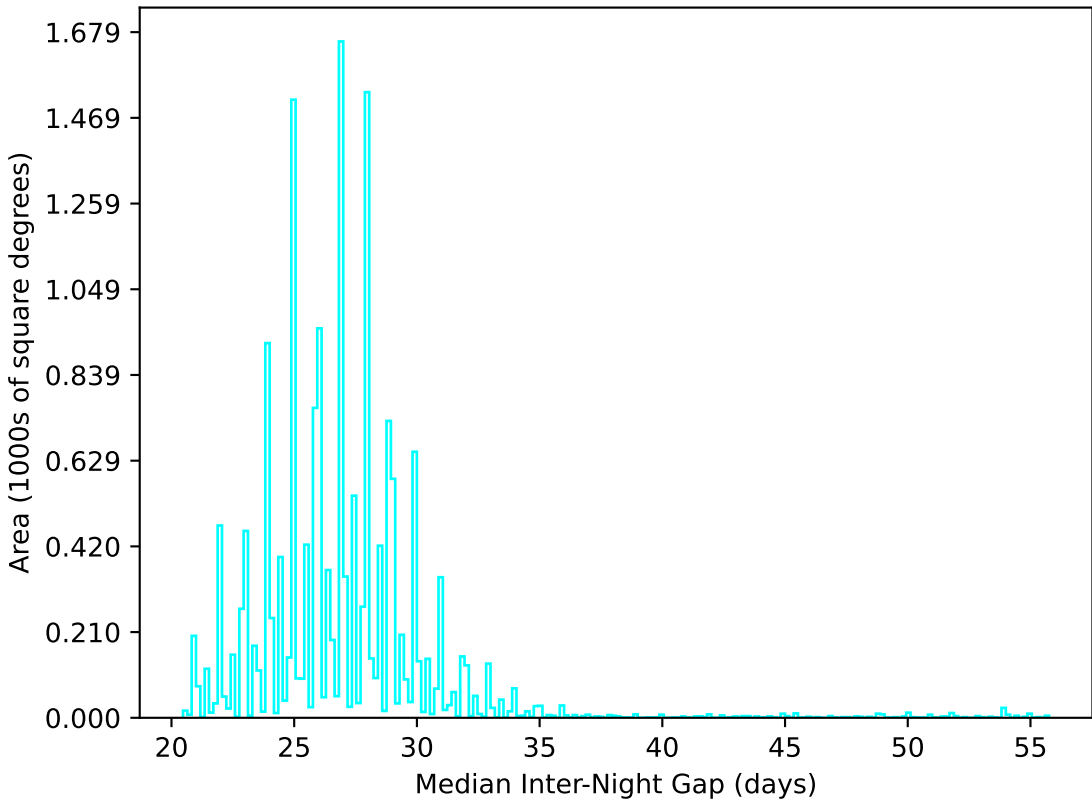
roll_pause_mjdp120_v3.4_10yrs WFD u band: Median Inter-Night Gap
