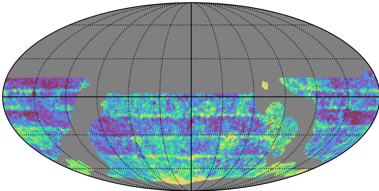
roll_pause_mjdp120_v3.4_10yrs WFD r band: Median Inter-Night Gap
