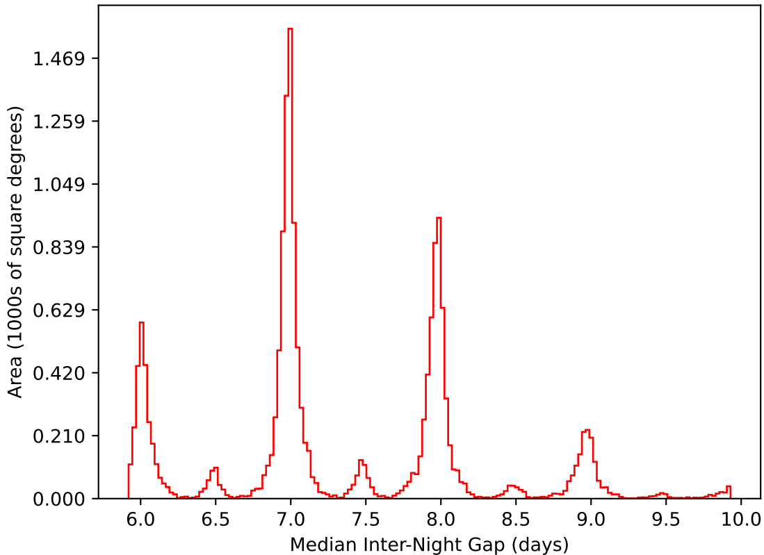
roll_pause_mjdp120_v3.4_10yrs WFD i band: Median Inter-Night Gap
