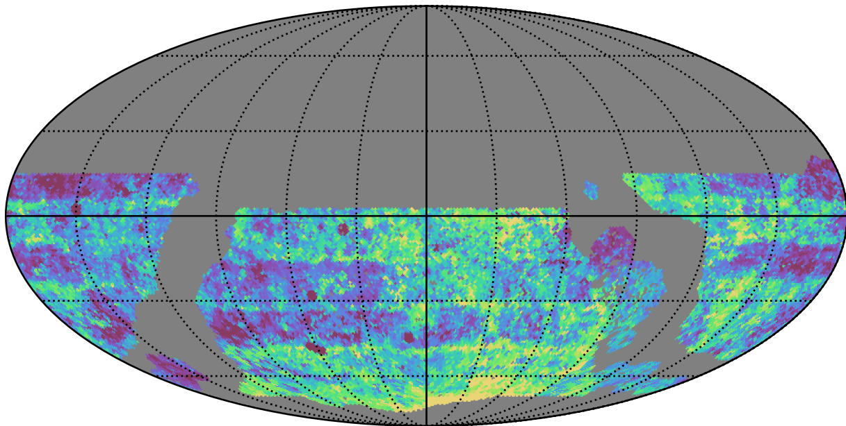
roll_pause_mjdp120_v3.4_10yrs WFD g band: Median Inter-Night Gap
