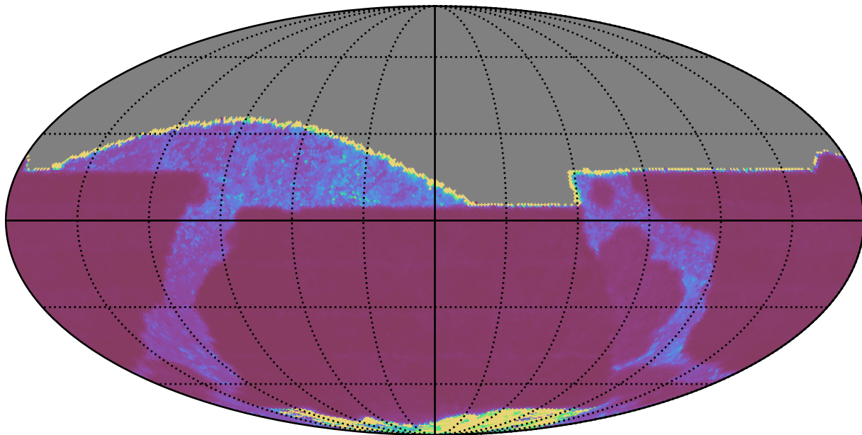
roll_pause_mjdp120_v3.4_10yrs All sky z band: Median Inter-Night Gap
