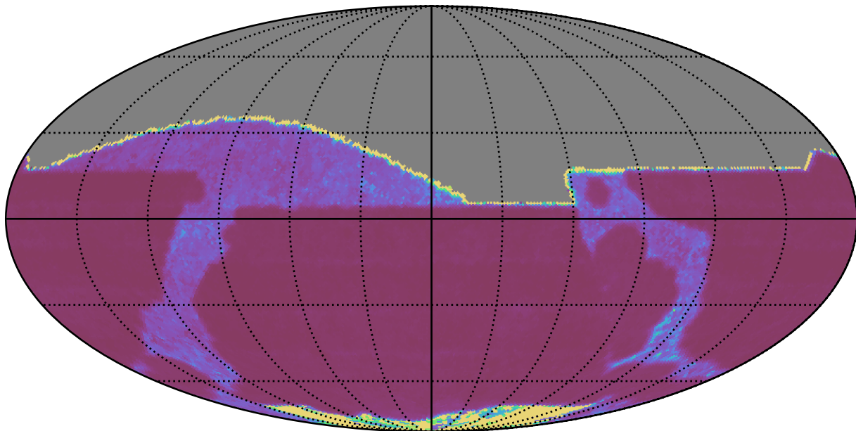
roll_pause_mjdp120_v3.4_10yrs All sky r band: Median Inter-Night Gap
