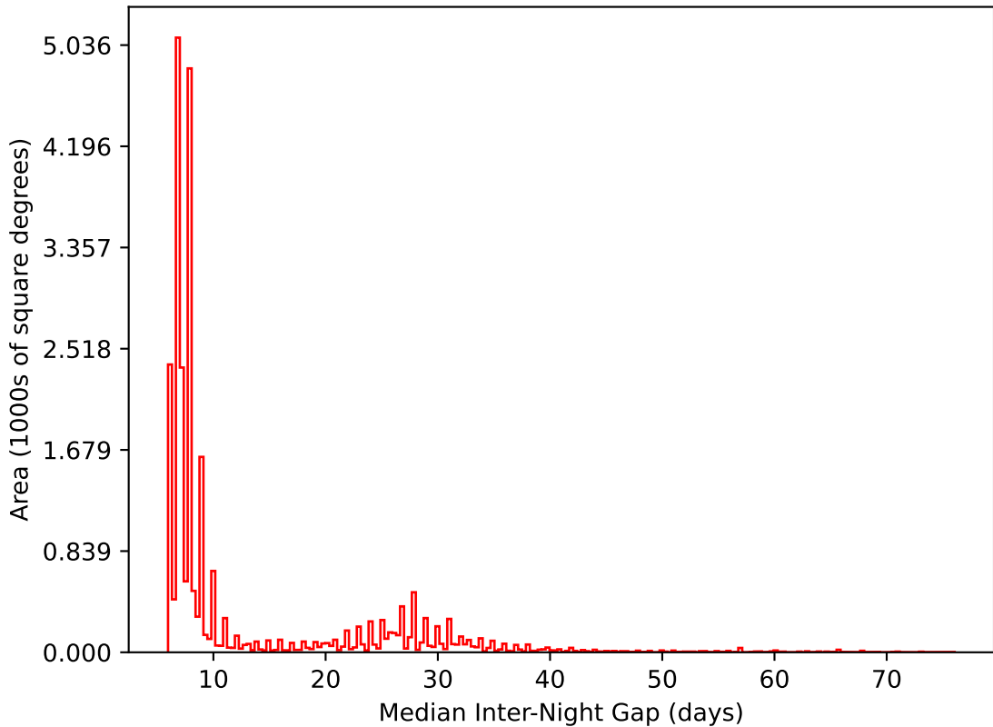
roll_pause_mjdp120_v3.4_10yrs All sky i band: Median Inter-Night Gap
