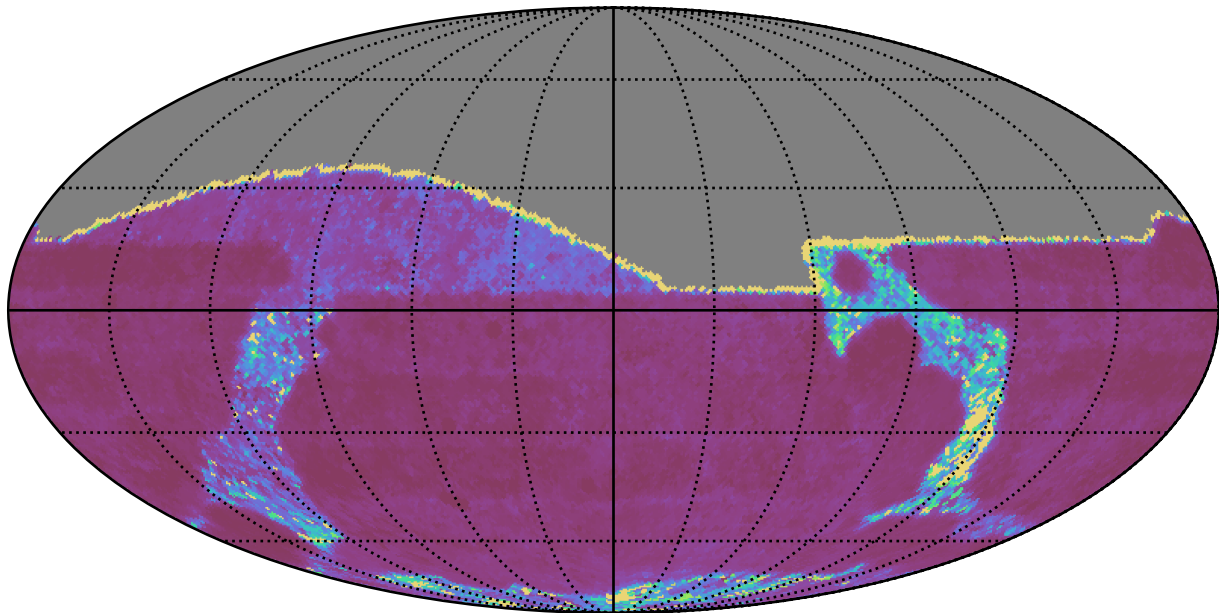
roll_pause_mjdp120_v3.4_10yrs All sky g band: Median Inter-Night Gap
