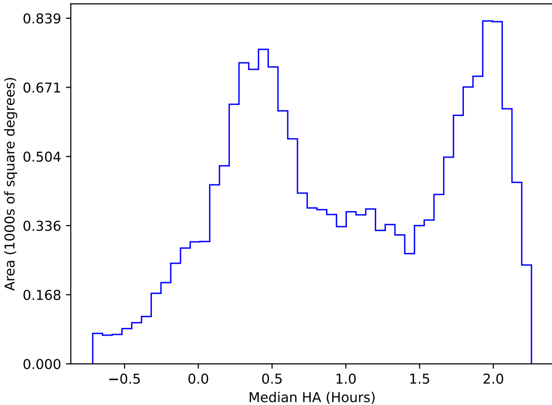
roll_pause_mjdp120_v3.4_10yrs WFD z band: Median HA
