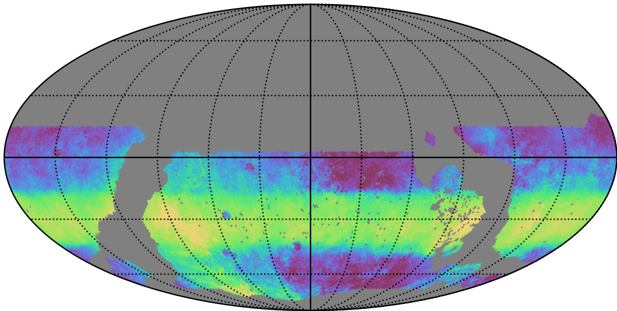
roll_pause_mjdp120_v3.4_10yrs WFD y band: Median HA
