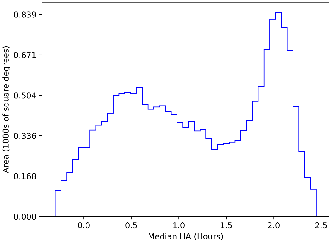
roll_pause_mjdp120_v3.4_10yrs WFD y band: Median HA
