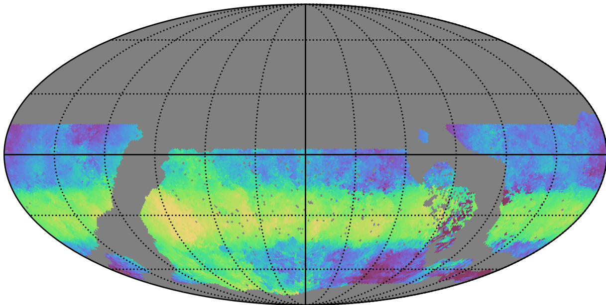
roll_pause_mjdp120_v3.4_10yrs WFD u band: Median HA
