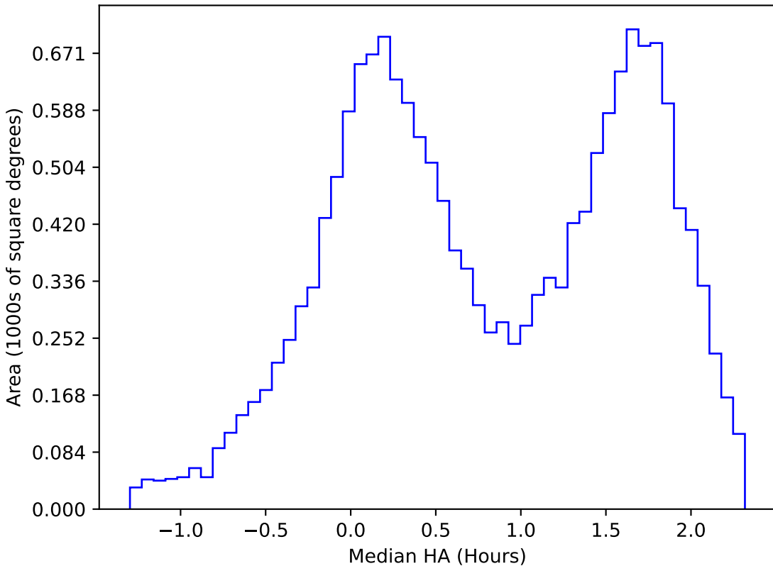
roll_pause_mjdp120_v3.4_10yrs WFD u band: Median HA
