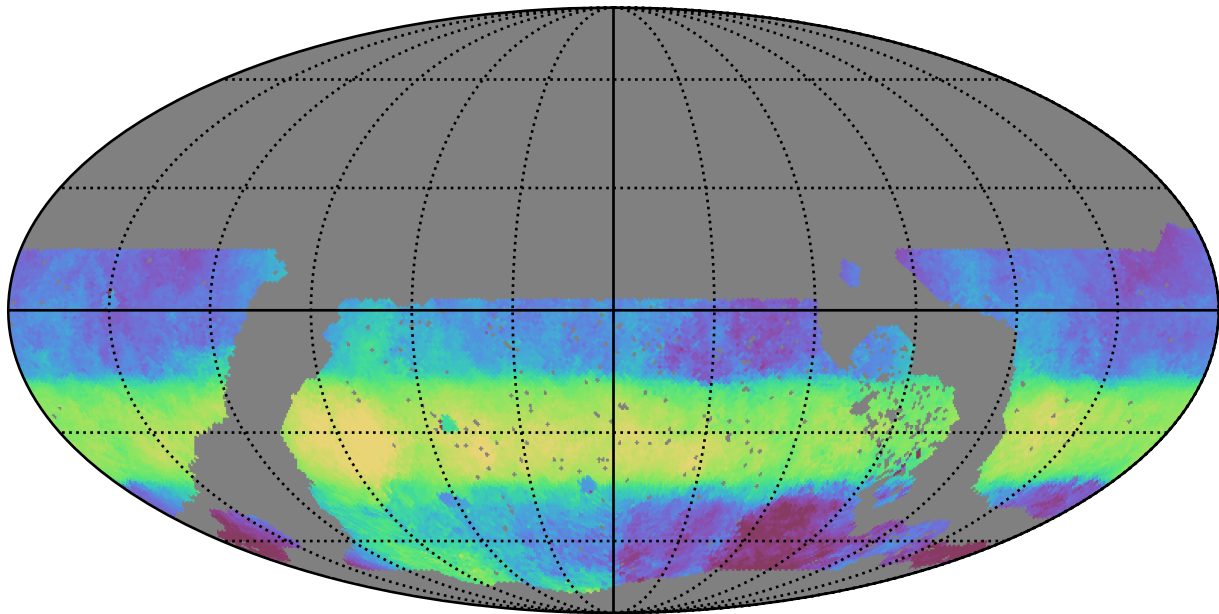
roll_pause_mjdp120_v3.4_10yrs WFD r band: Median HA
