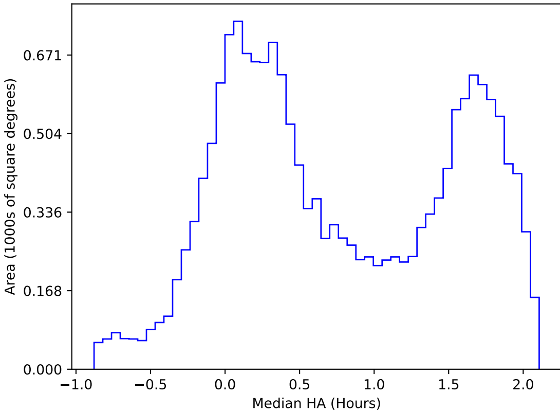
roll_pause_mjdp120_v3.4_10yrs WFD r band: Median HA
