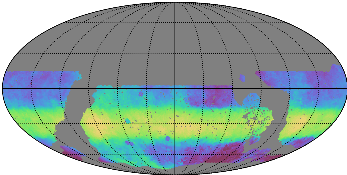
roll_pause_mjdp120_v3.4_10yrs WFD i band: Median HA
