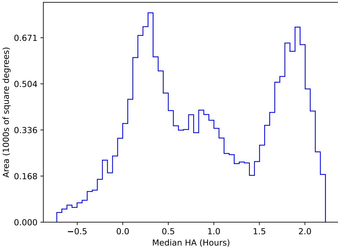
roll_pause_mjdp120_v3.4_10yrs WFD i band: Median HA
