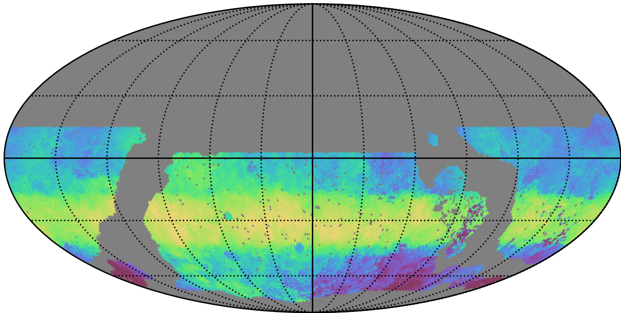
roll_pause_mjdp120_v3.4_10yrs WFD g band: Median HA
