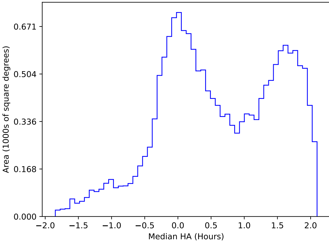
roll_pause_mjdp120_v3.4_10yrs WFD g band: Median HA
