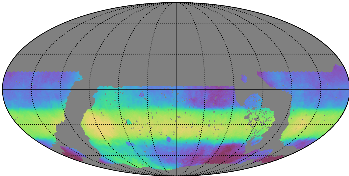
roll_pause_mjdp120_v3.4_10yrs WFD all bands: Median HA
