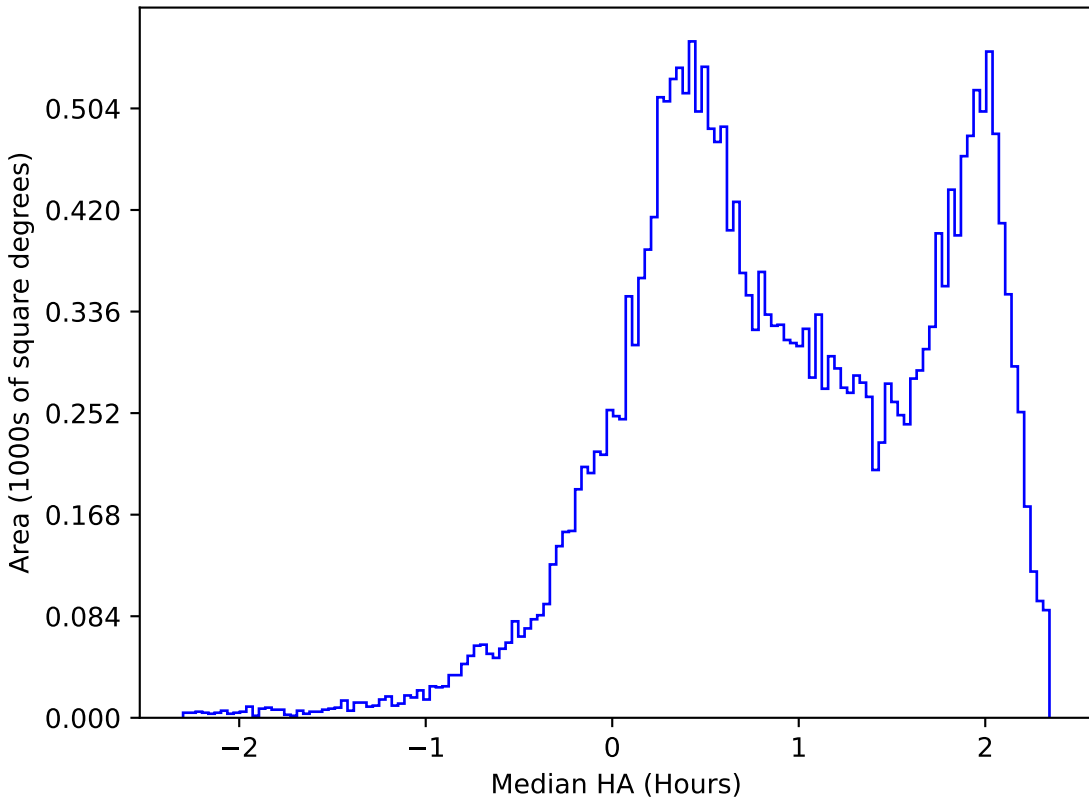
roll_pause_mjdp120_v3.4_10yrs All sky z band: Median HA
