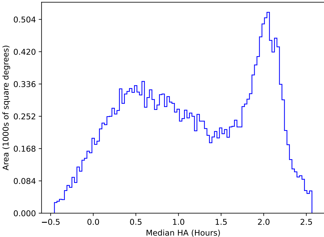
roll_pause_mjdp120_v3.4_10yrs All sky y band: Median HA
