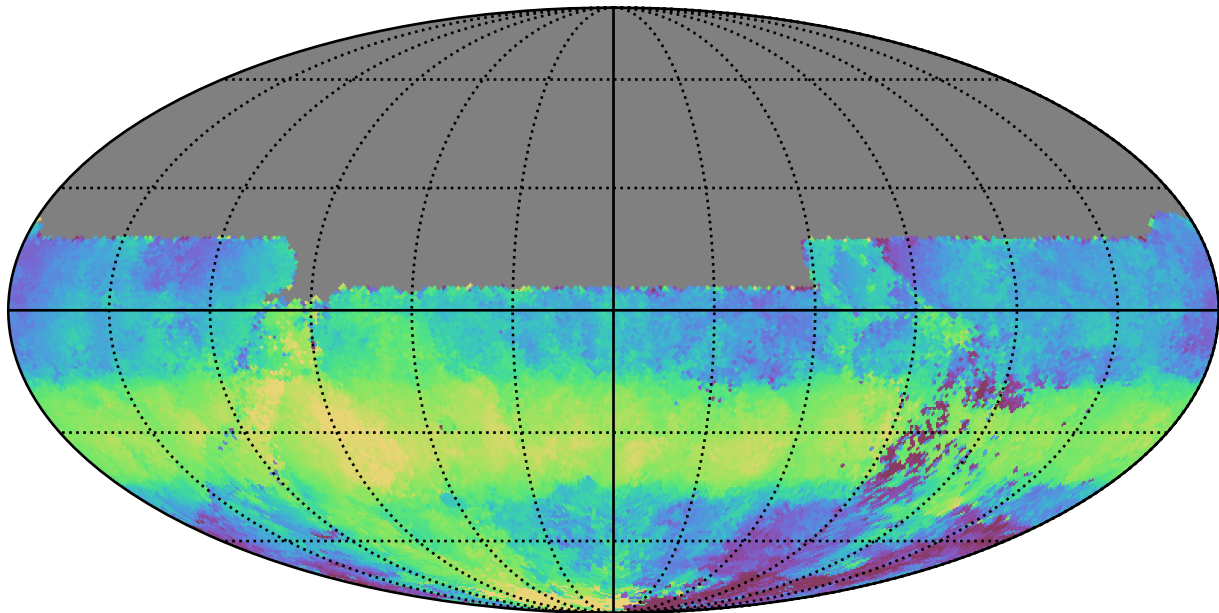
roll_pause_mjdp120_v3.4_10yrs All sky u band: Median HA
