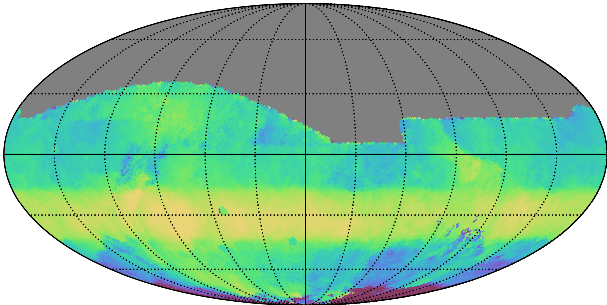
roll_pause_mjdp120_v3.4_10yrs All sky r band: Median HA
