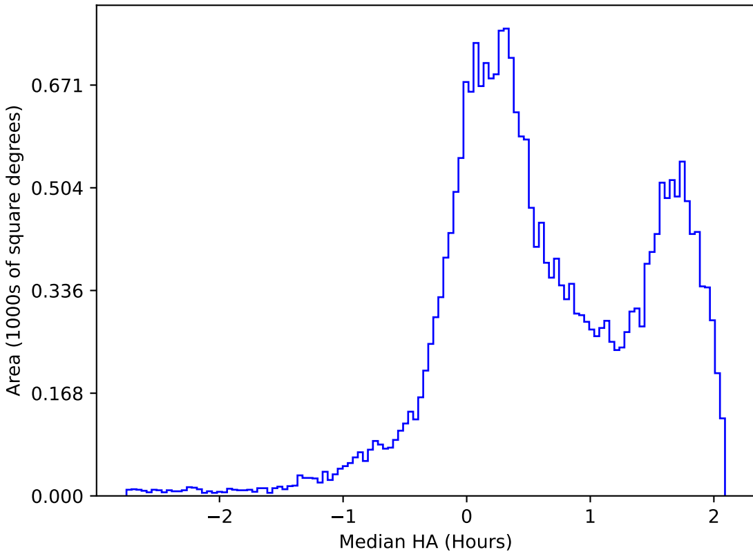
roll_pause_mjdp120_v3.4_10yrs All sky r band: Median HA
