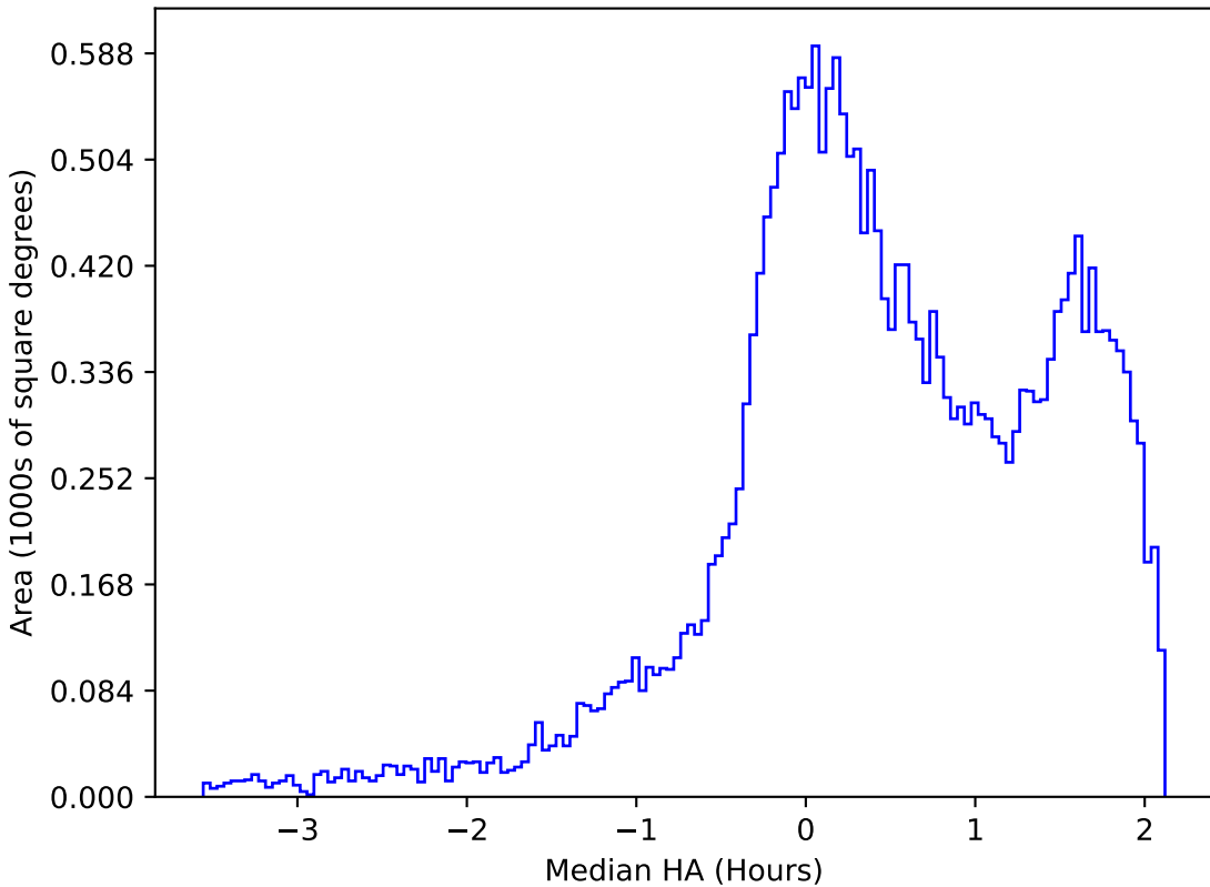
roll_pause_mjdp120_v3.4_10yrs All sky g band: Median HA
