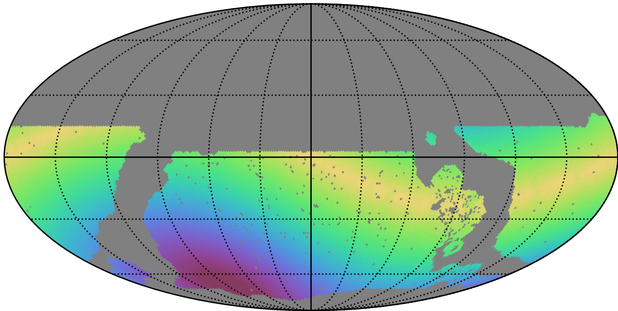
roll_pause_mjdp120_v3.4_10yrs WFD y band: Max solarElong
