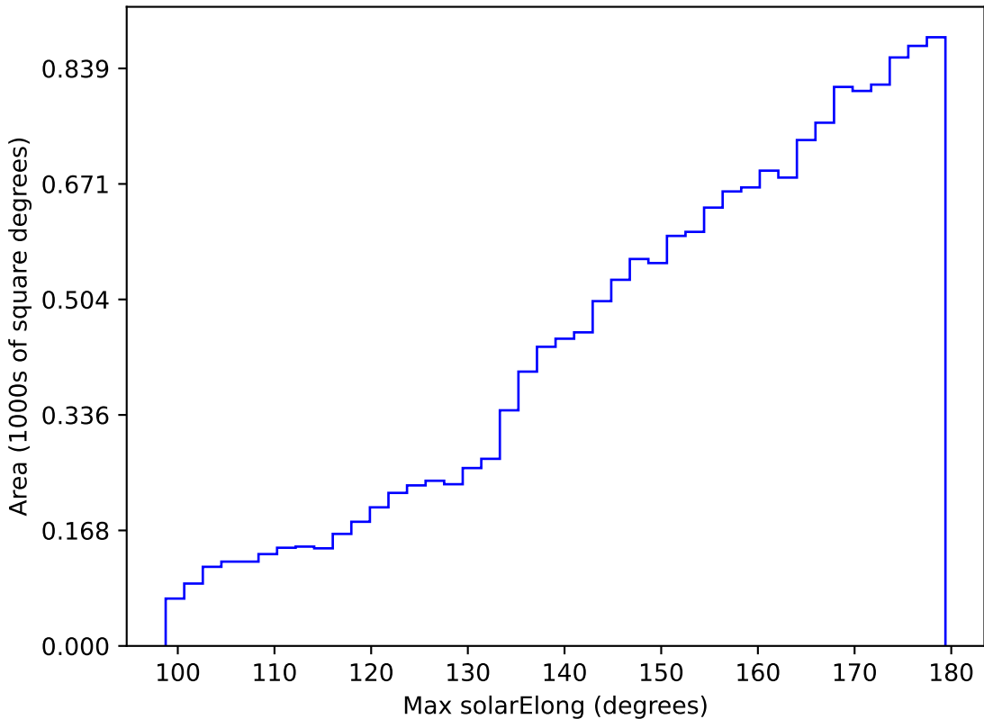
roll_pause_mjdp120_v3.4_10yrs WFD y band: Max solarElong
